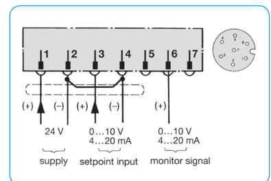
connection diagram for supply and signal
